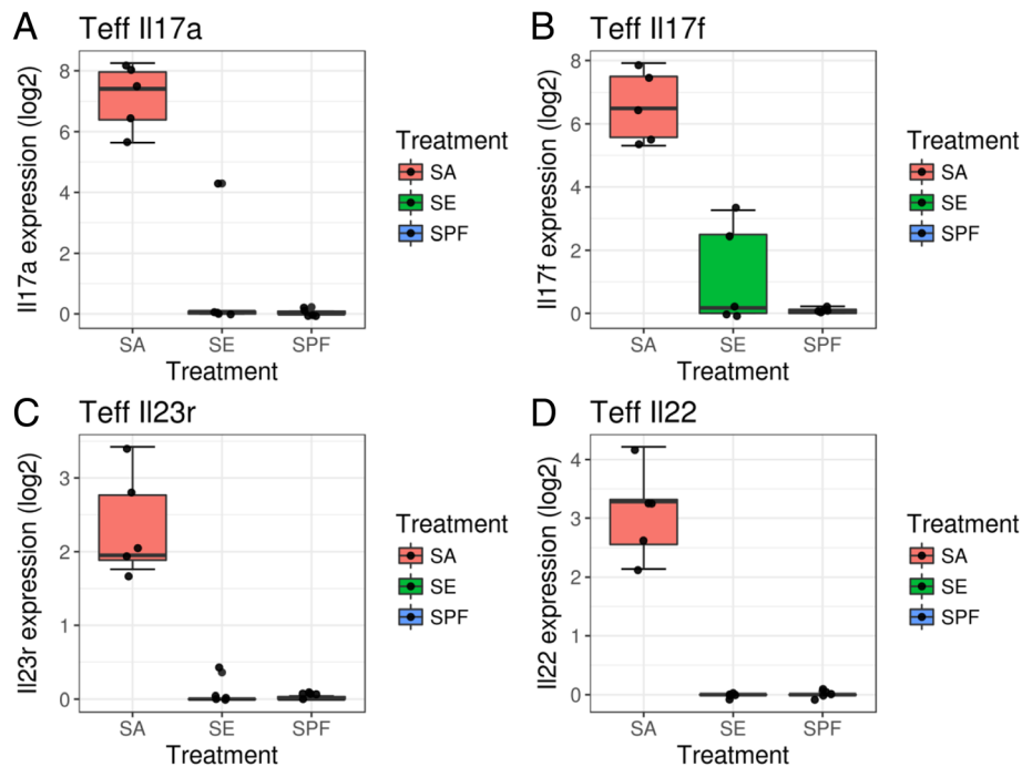
Fig. 5 Staphylococcus aureus exposure triggers Th17 response in effector T cells. mRNA expression ( \log_2 FPKM) of cutaneous effector T cells from specific pathogen-free (SPF) mice colonized with Staphylococcus aureus (SA), Staphylococcus epidermidis (SE), or none (SPF). Compared to the SPF control, the Staphylococcus aureus colonization triggers gene expression in a IL-17A (adj p value = 3.51e-7 ), b IL-17F (adj p value = 3.08e-6 ), c IL-23R (adj p value = 3.74e-8 ), and d IL-22 (adj p value = 1.01e09 ). Colonization with Staphylococcus epidermidis does not trigger Th17 response
